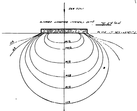
Pressure bulb for 256-ton load on raft foundation (16-ft. by 16-ft. base).
